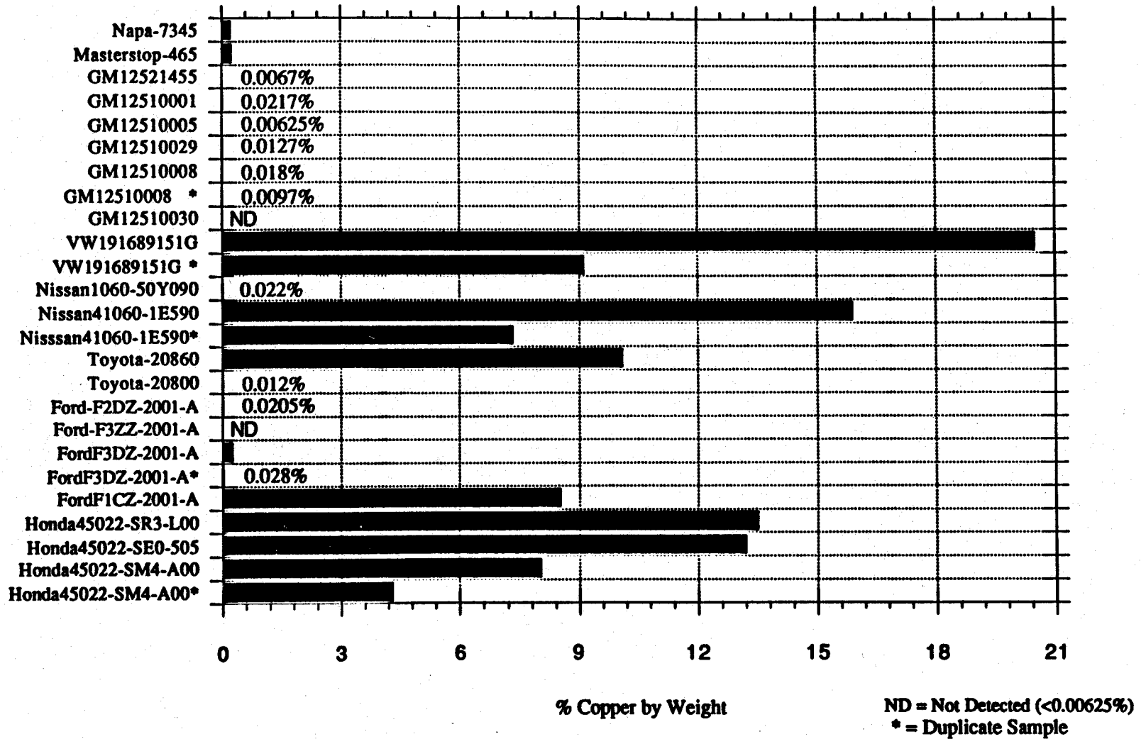
Figure 2: Total Copper in Brake Pads
