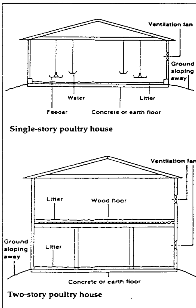
Figure 1.—Two types of litter-floor poultry houses.
