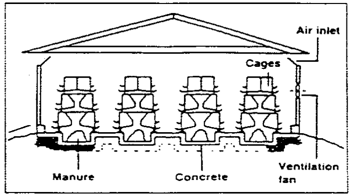
Figure 1.—Shallow-pit poultry house with cages.
