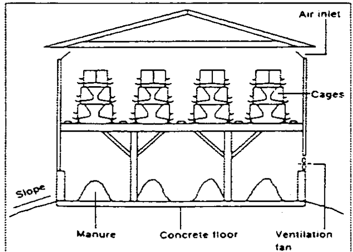
Figure 2.—High-rise poultry house with cages.
