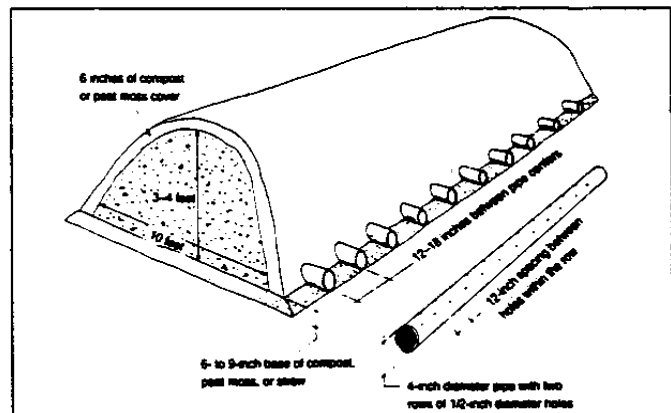
Figure 3.—Passively aerated windrow method for composting manure.
