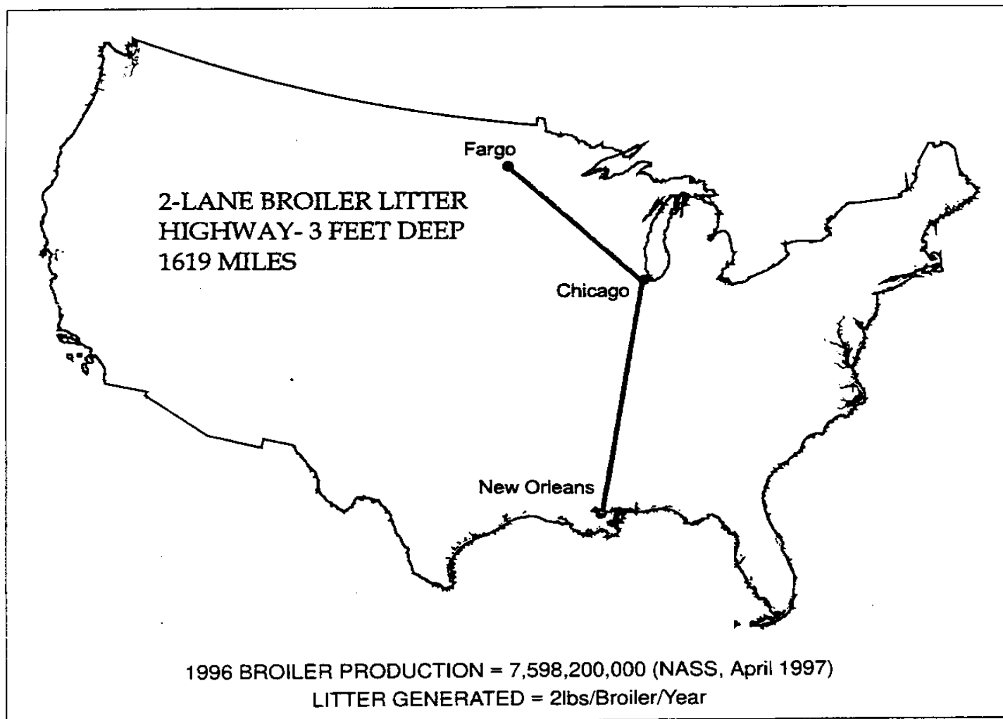
Figure 1.—The broiler litter highway: broiler litter generated in 1996, in the United States.
