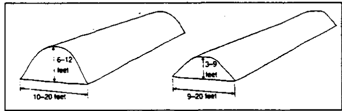
Figure 1.—Typical windrow shapes and dimensions.
