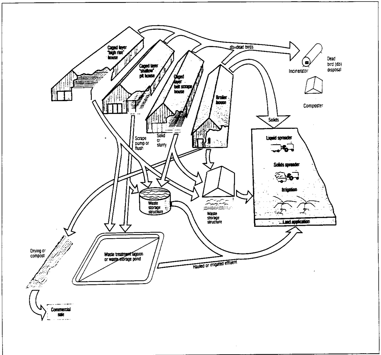
Figure 1.—Representative components of a poultry waste management system.
